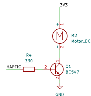
Haptics – using motor and transistor
