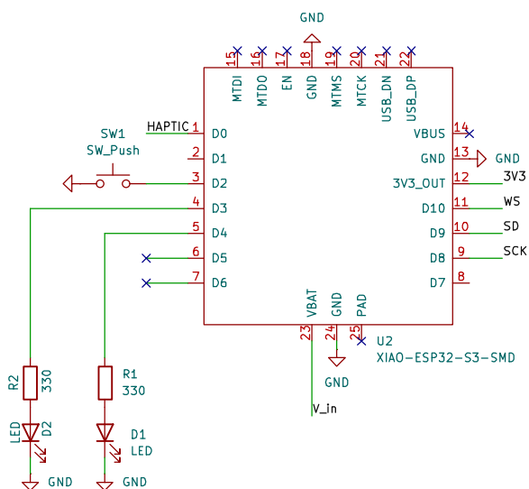
Seed Xiao and basic GPIO
